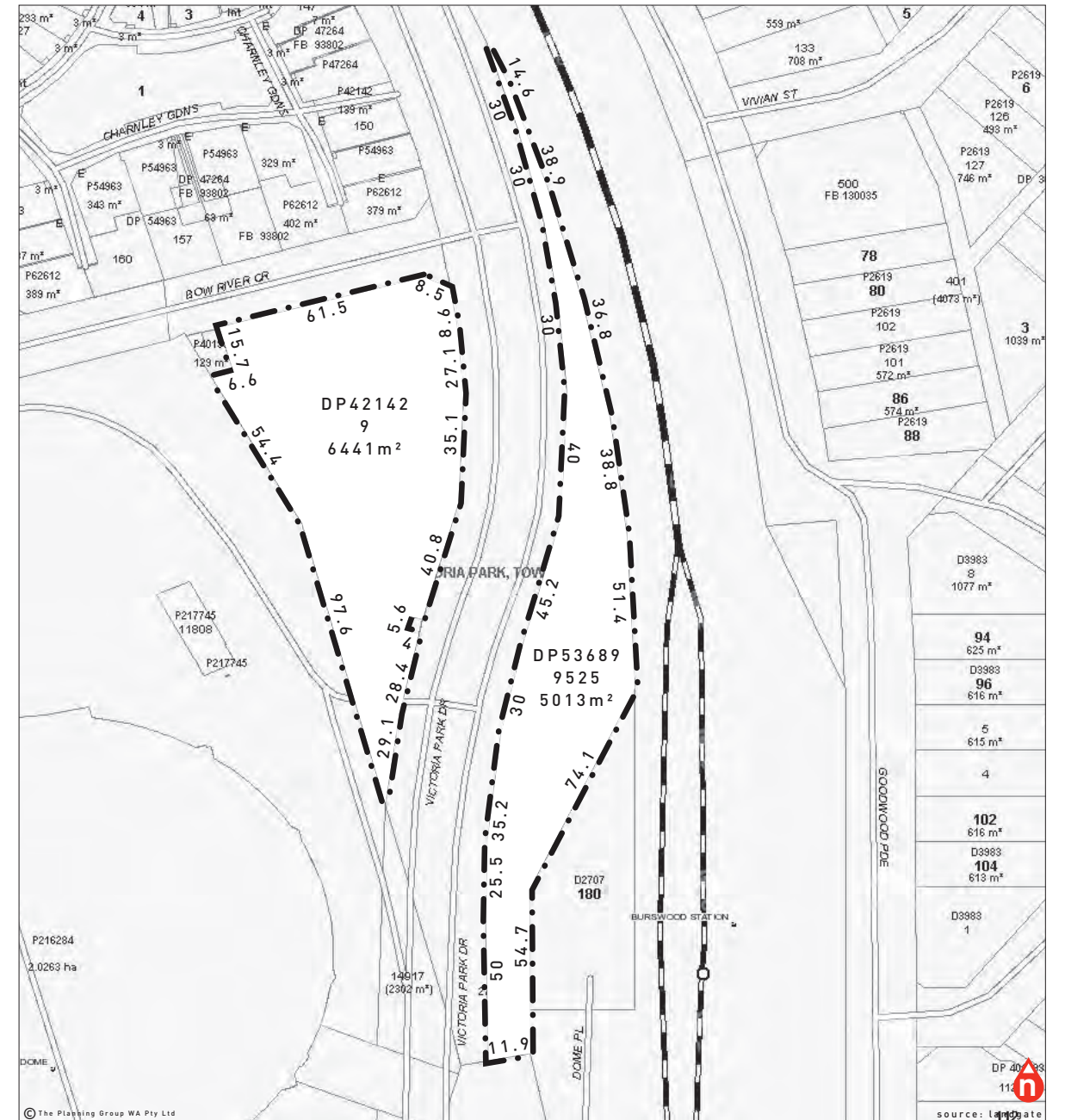
Figure 2. Site Plan
